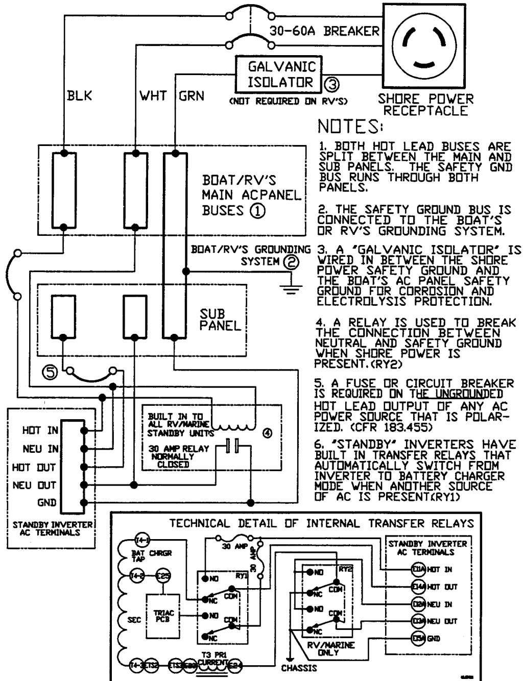
Figure 10, Polarized System for Marine Installations
