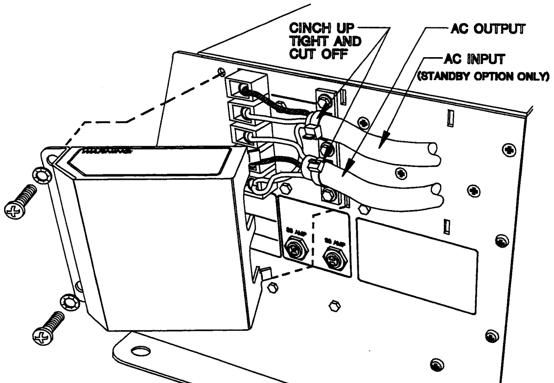
Figure 5, Hardwire Terminal
